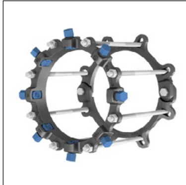
Stargrip® series 3100P for Ductile Iron Pipe
