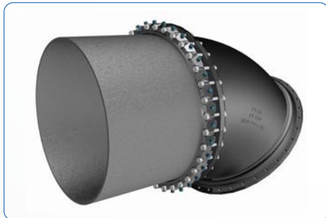
SERIES 3000 STARGRIP RESTRAINTS (For Ductile Iron Pipe) 54" AND 60"
