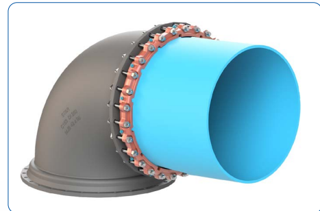
SERIES 4000 STARGRIP RESTRAINTS (For PVC Pipe) 42" AND 48"
