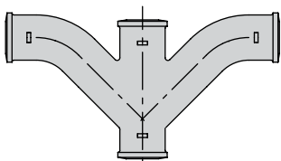
Double Combination Wye & 1/8" Bend
