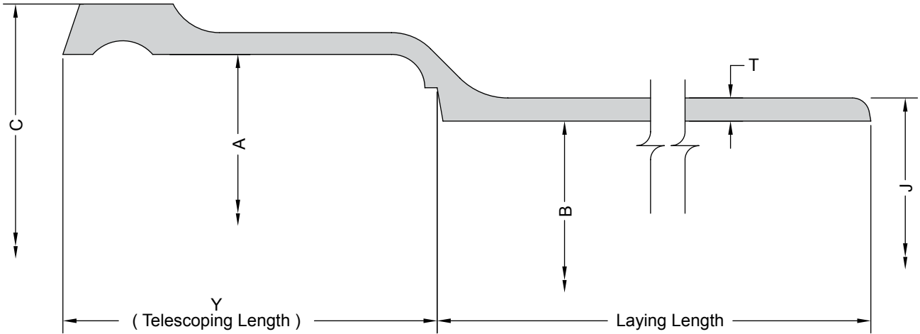
DETAILS OF HUB & SPIGOT FOR SV*
